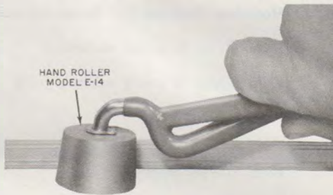
Fig. 2—Applying Roller to Wire Run
