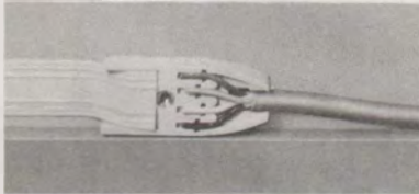
Fig. 7—Terminating Wire in No. 721 Transition
