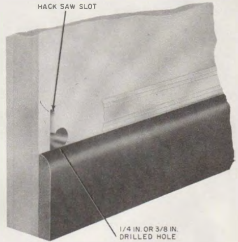
Fig. 11—Hole Through Wall for B Station Wire
