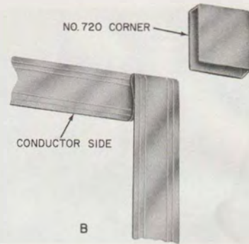
Fig. 3—90-Degree Turn in B Station Wire
